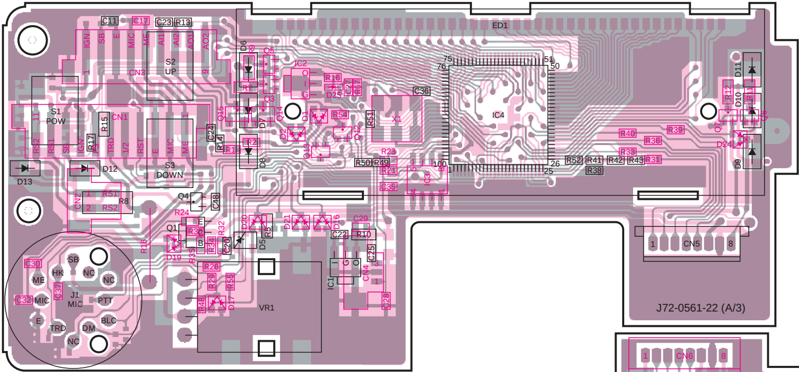
DISPLAY UNIT (X54-3190-20) Component side view : KCH-10
