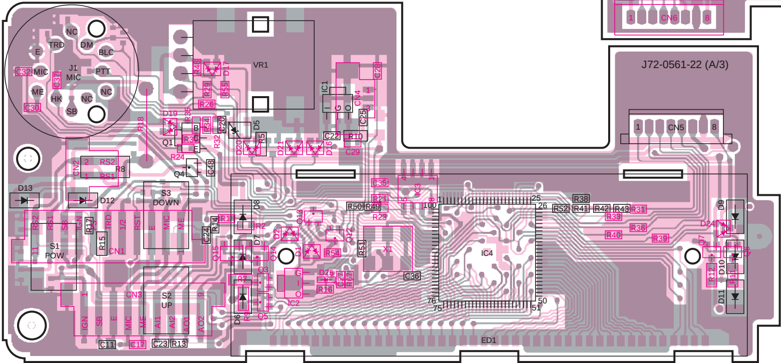
DISPLAY UNIT (X54-3190-20) Foil side view : KCH-10
